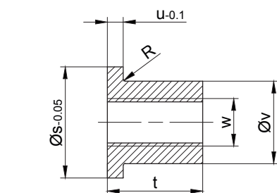
Pos.3 Sleeve
