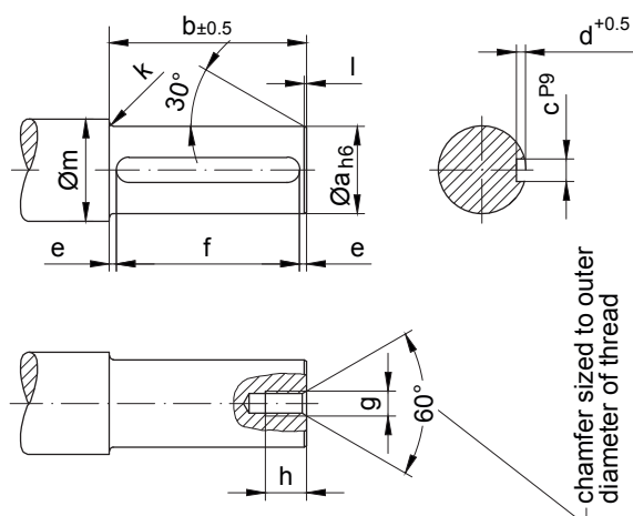
Pos.1 Shaft
