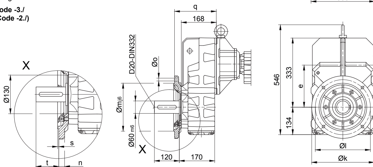
Flange dimensions
