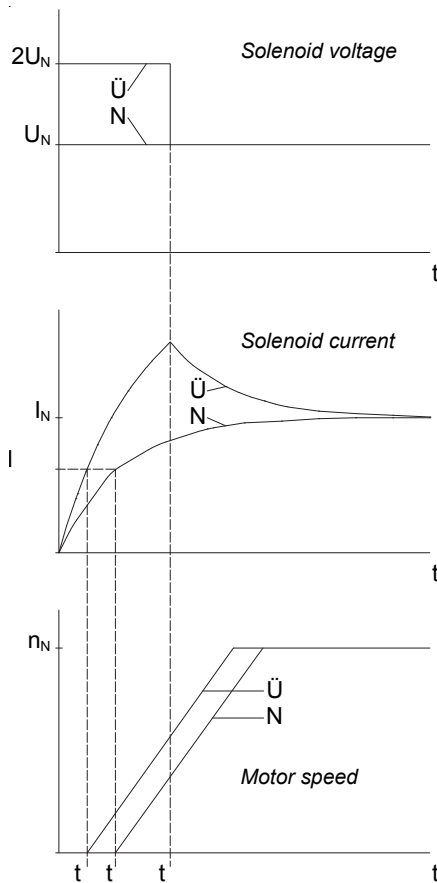
Figure 3: Idealised curves of coil voltage, coil current and motor speed with normal excitation (N) and overexcitation (Ü). t_{0U} : overexcitation time; t_{AN} , t_{AU} : Response time with normal excitation and overexcitation.
