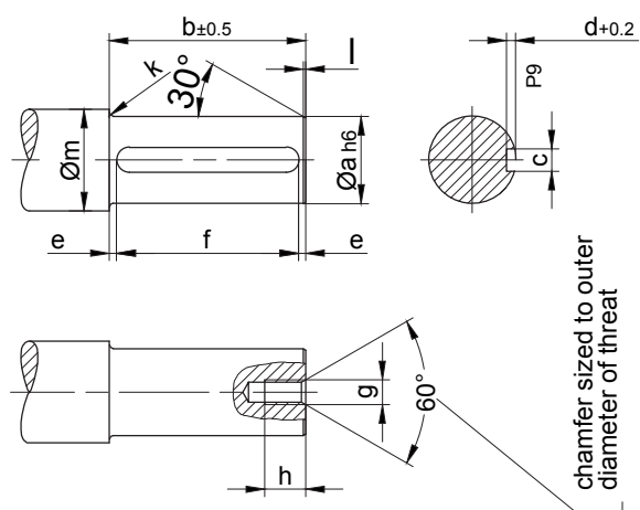
Pos.1 Shaft
