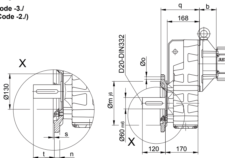
Flange dimensions
