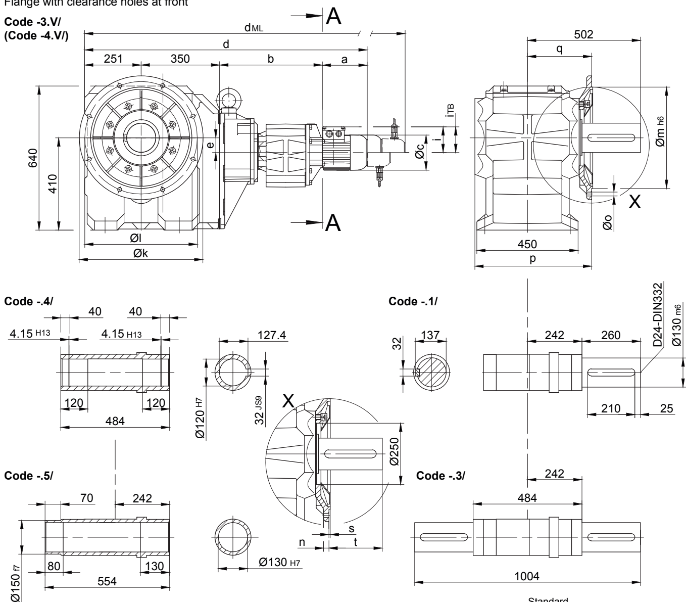
Flange dimensions
