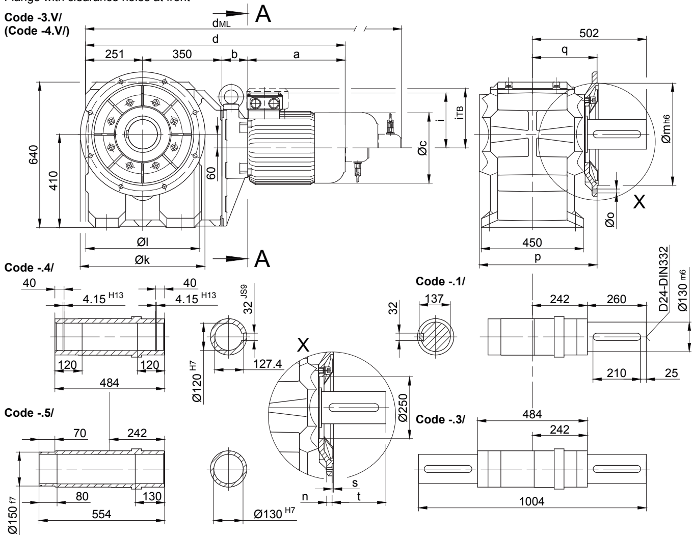
Flange dimensions
