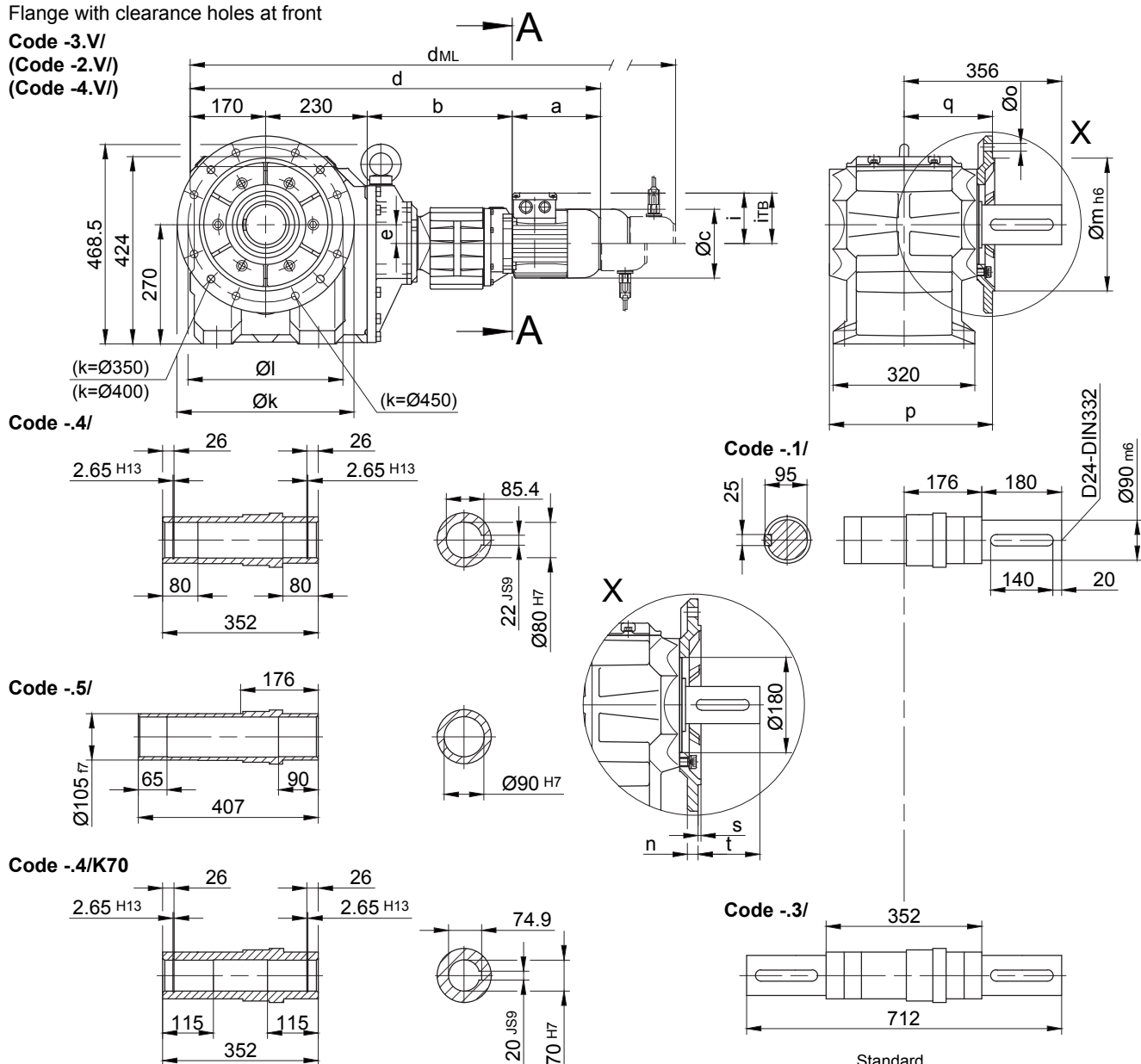
Flange dimensions
