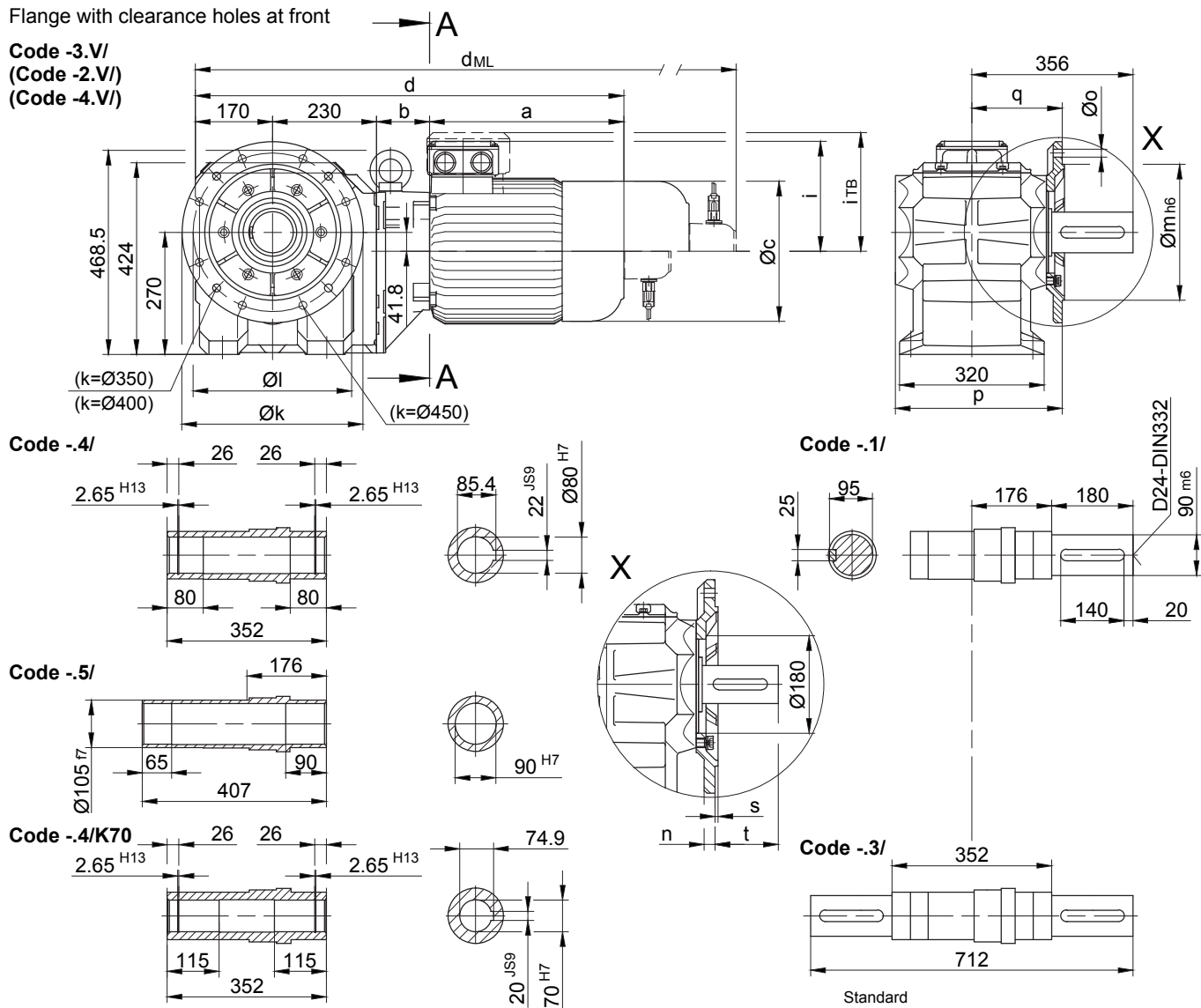
Flange dimensions
