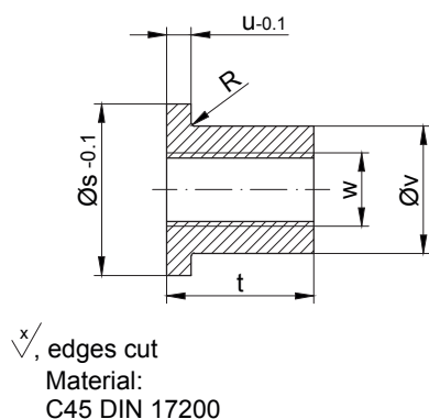
Pos.3 Sleeve
