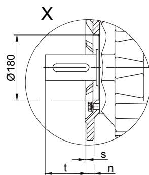
Flange dimensions
