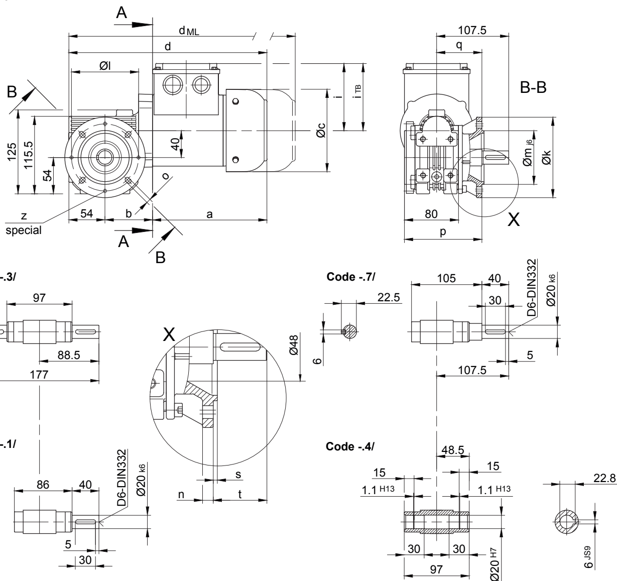
Flange dimensions
