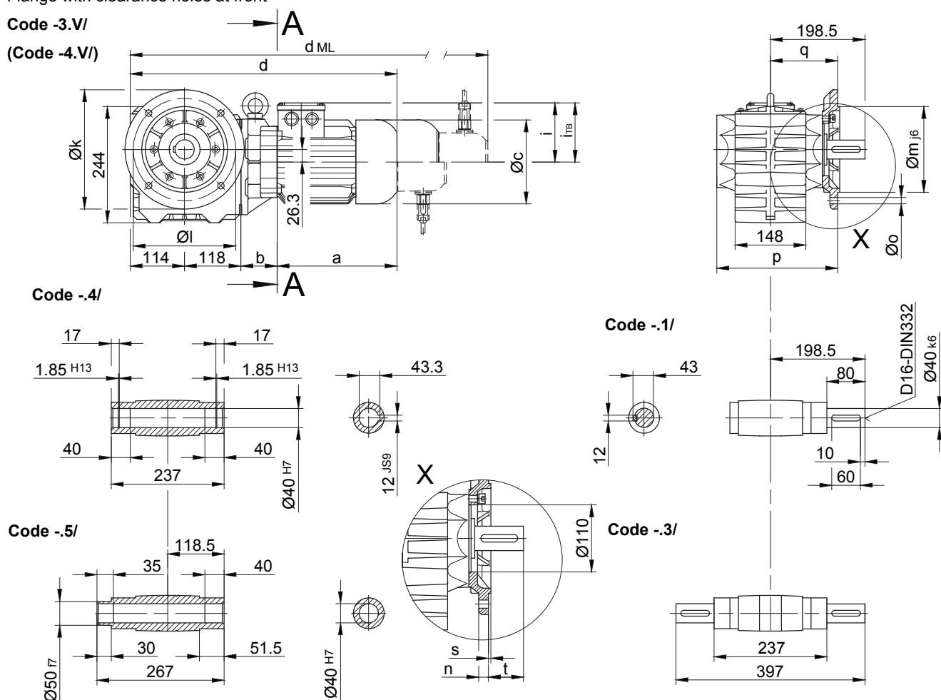
Flange dimensions
